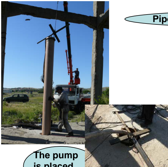
Lowering the submersible pump through a 6m long pipe for the second test, May (28-30)
